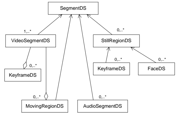
Figure 3. Definition of segment types, through the inheritance mechanism.
