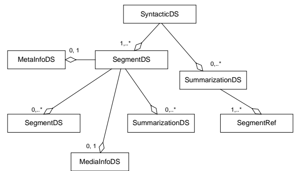
Figure 2. Structure of the audiovisual material in SyntacticDS.
