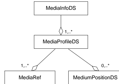
Figure 6. Media storage information and profiles in MediaInfoDS.
