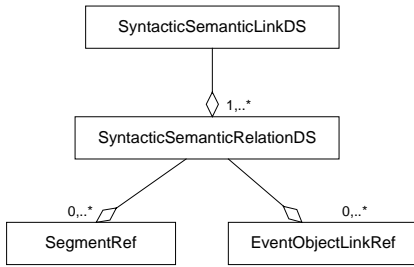
Figure 5. Linking between syntactic and semantic information.
